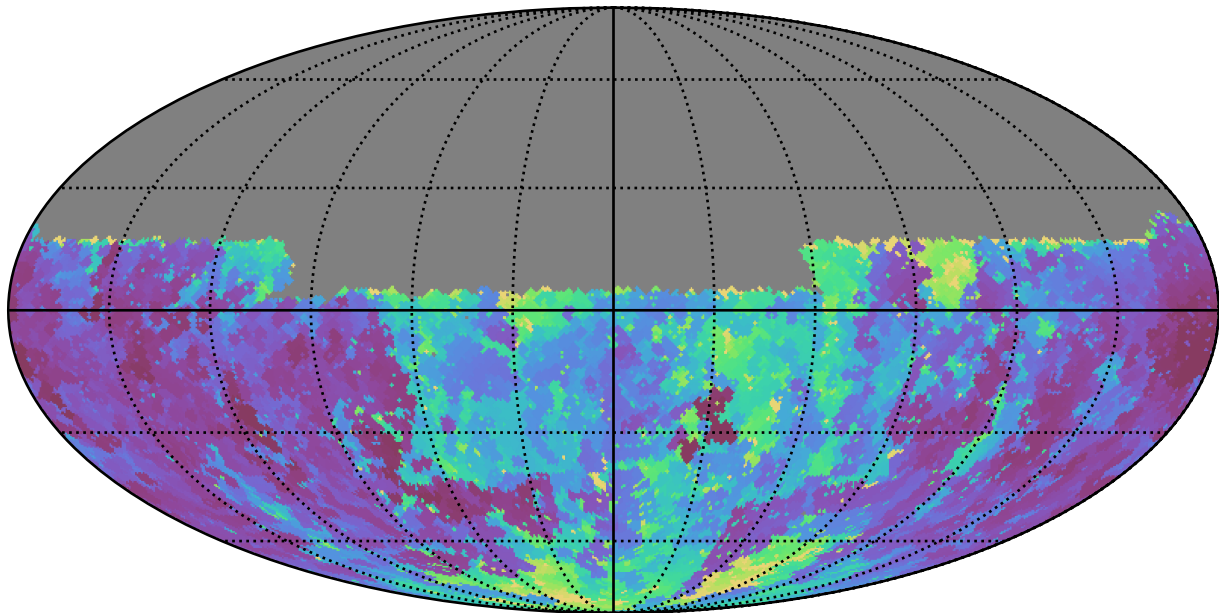
too_10_4v3.4_10yrs Yr 1 u band: Min seeingGeom
