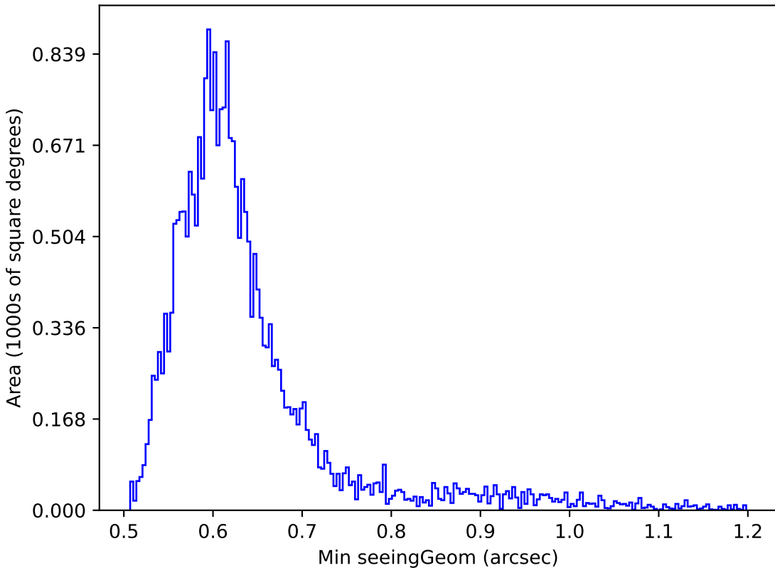
too_10_4v3.4_10yrs Yr 1 r band: Min seeingGeom
