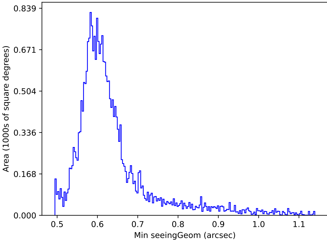
too_10_4v3.4_10yrs Yr 1 i band: Min seeingGeom
