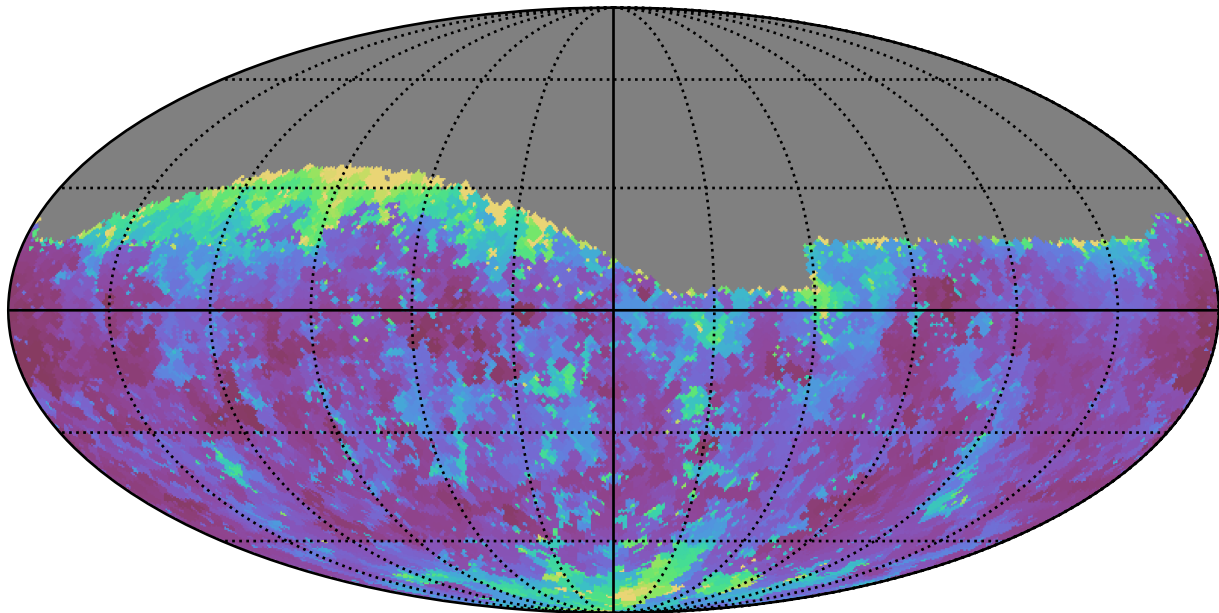
too_10_4v3.4_10yrs Yr 1 g band: Min seeingGeom
