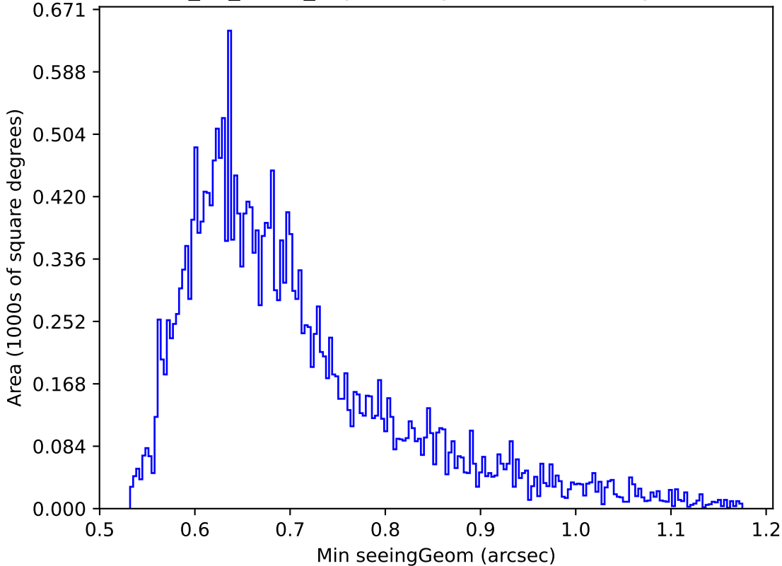
too_10_4v3.4_10yrs Yr 1 g band: Min seeingGeom
