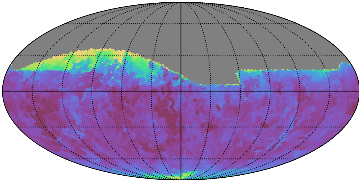
too_10_4v3.4_10yrs Yr 1 all bands: Min seeingGeom
