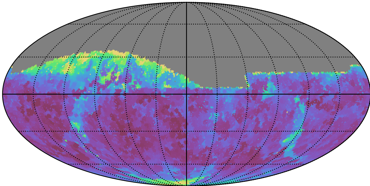
too_10_4v3.4_10yrs Yr 1 z band: Min seeingEff
