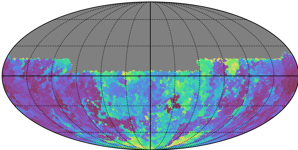
too_10_4v3.4_10yrs Yr 1 u band: Min seeingEff
