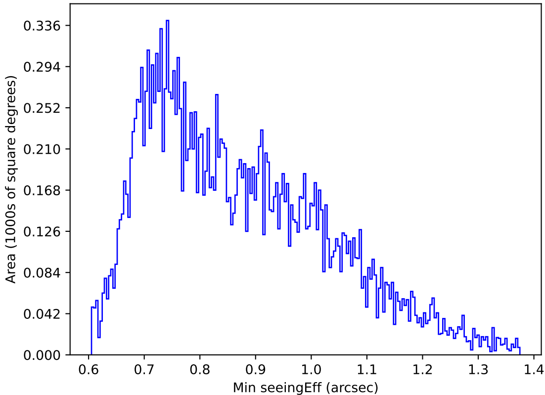
too_10_4v3.4_10yrs Yr 1 u band: Min seeingEff
