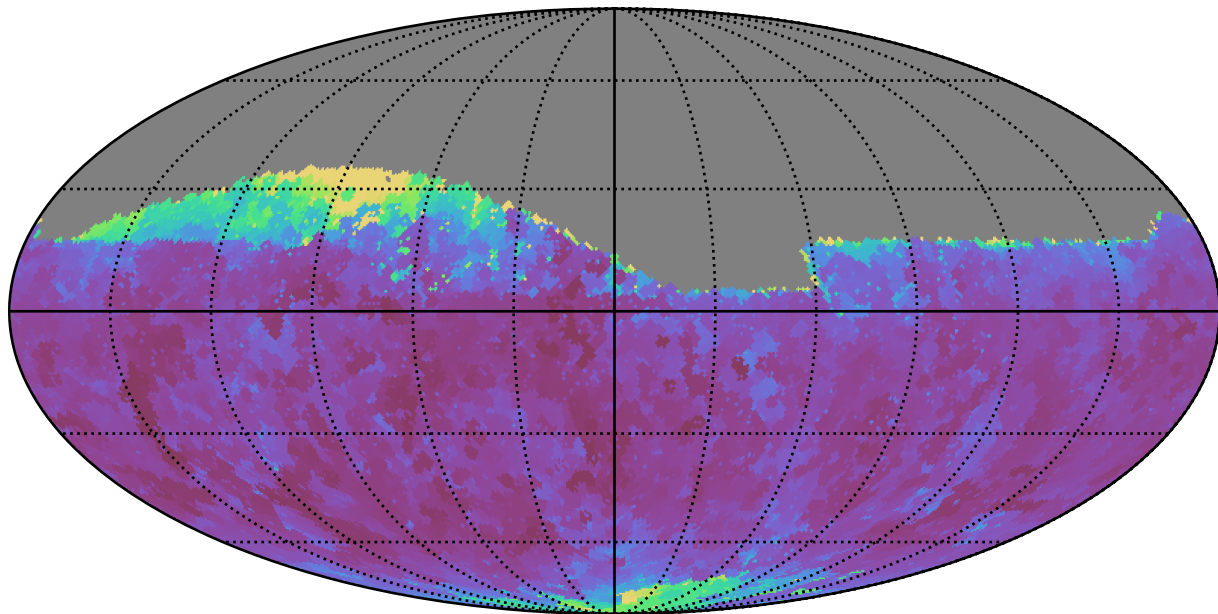
too_10_4v3.4_10yrs Yr 1 r band: Min seeingEff
