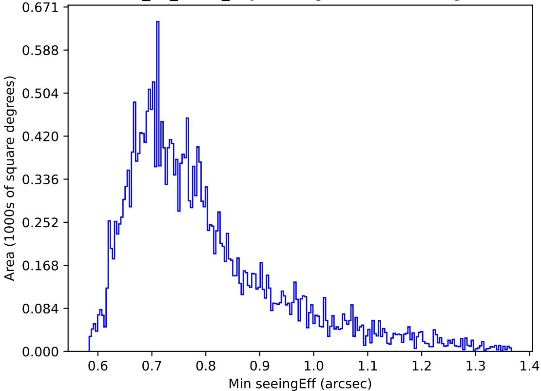
too_10_4v3.4_10yrs Yr 1 g band: Min seeingEff
