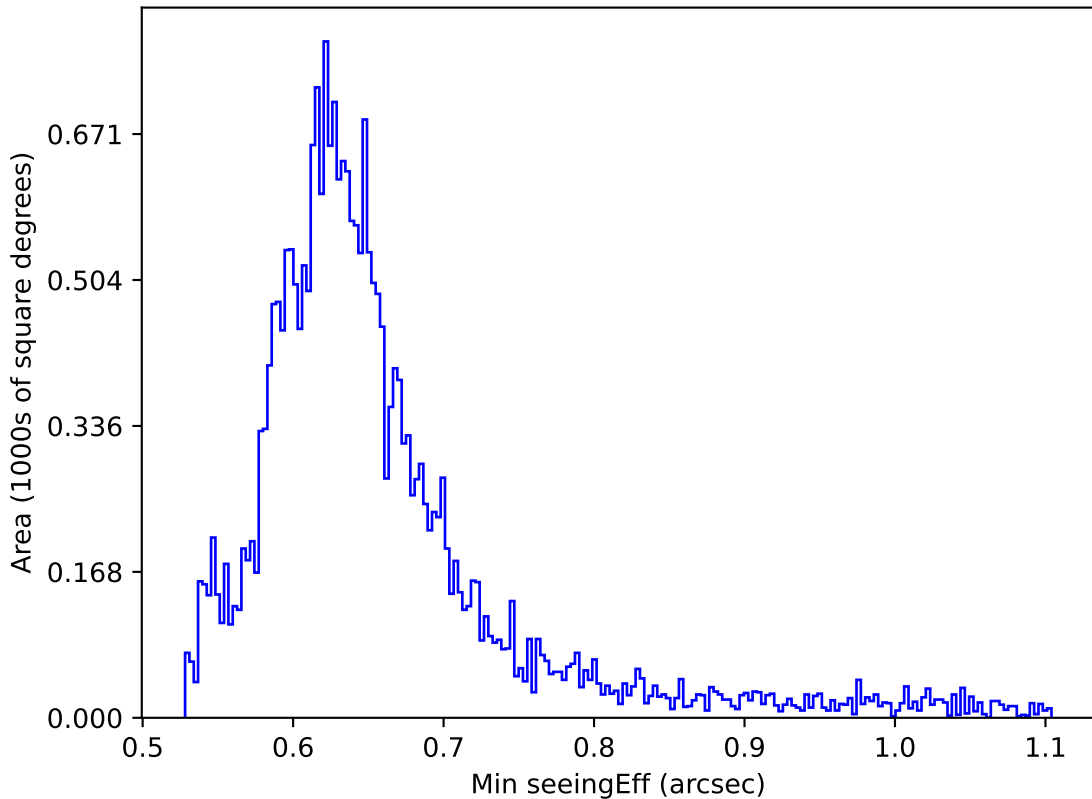
too_10_4v3.4_10yrs Yr 1 all bands: Min seeingEff
