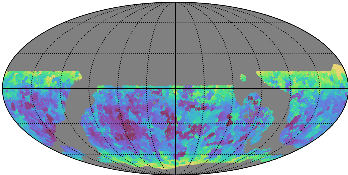
too_10_4v3.4_10yrs WFD z band: Min seeingEff
