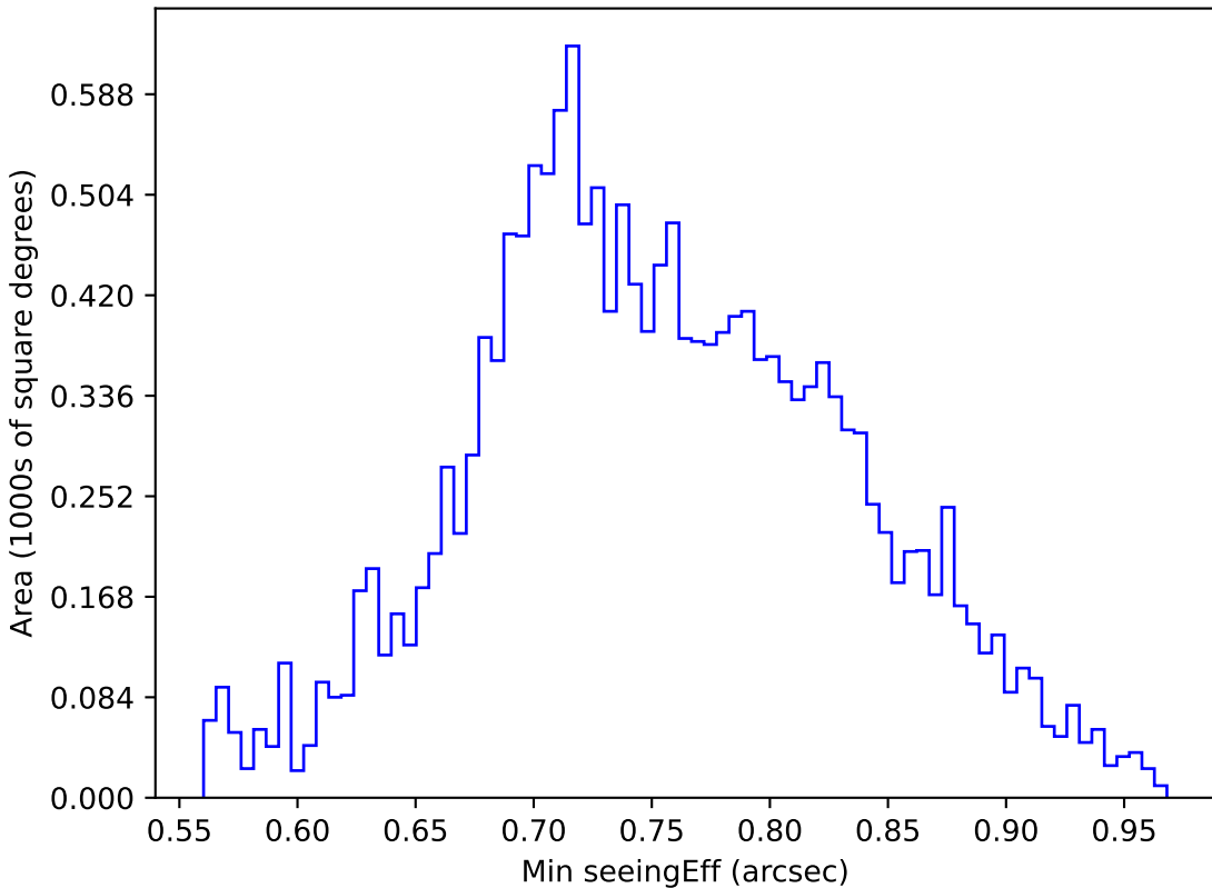
too_10_4v3.4_10yrs WFD u band: Min seeingEff
