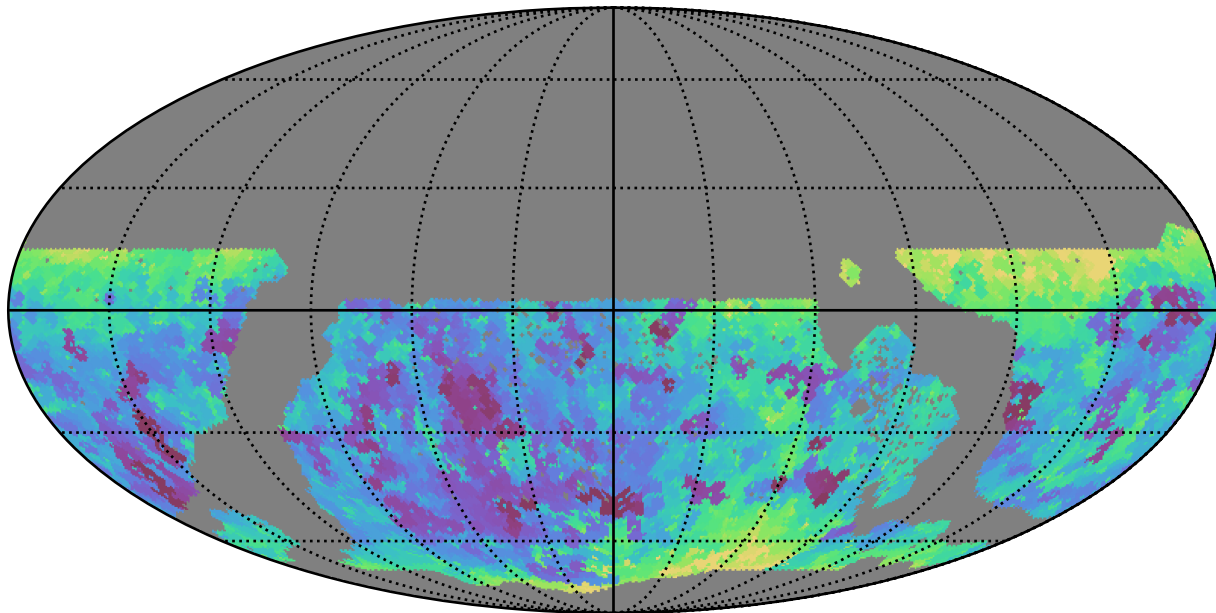
too_10_4v3.4_10yrs WFD r band: Min seeingEff
