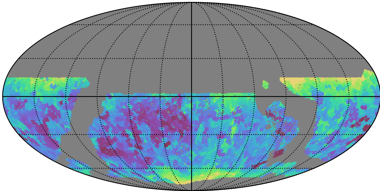
too_10_4v3.4_10yrs WFD i band: Min seeingEff
