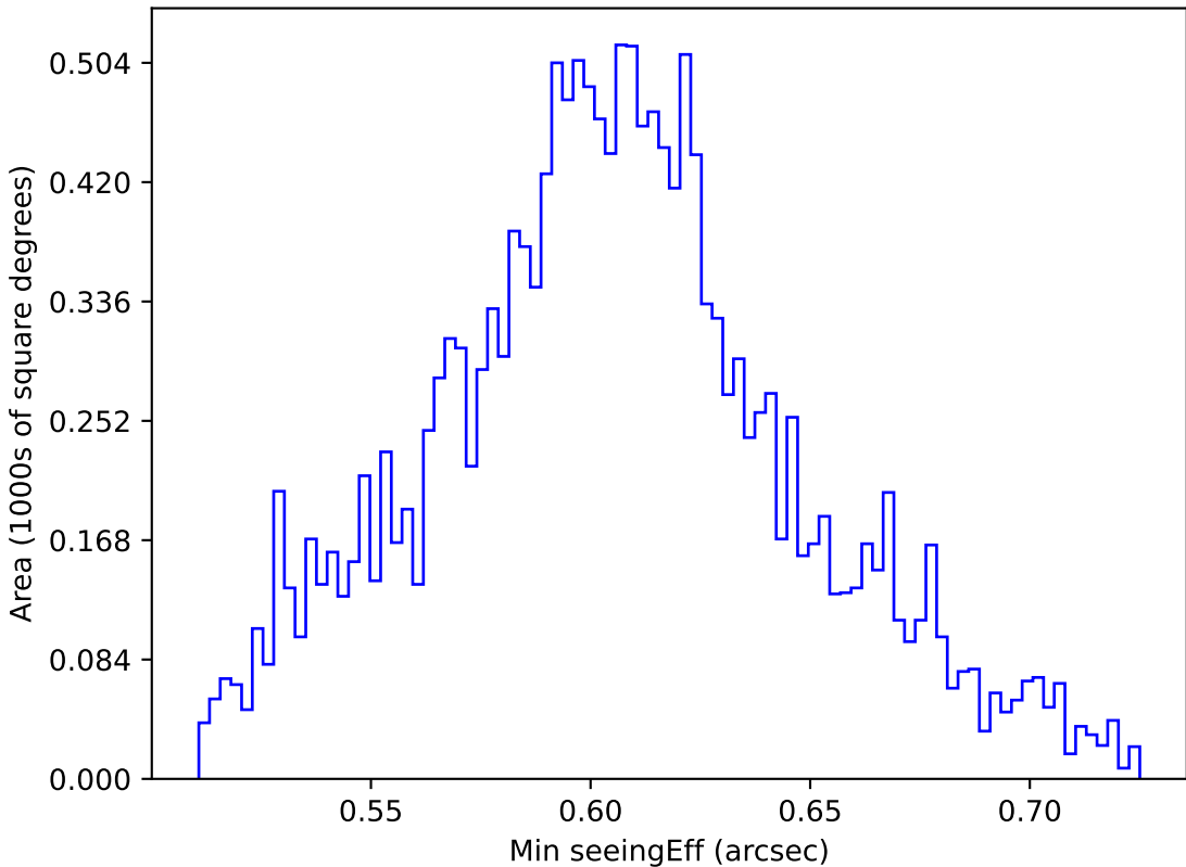
too_10_4v3.4_10yrs WFD i band: Min seeingEff
