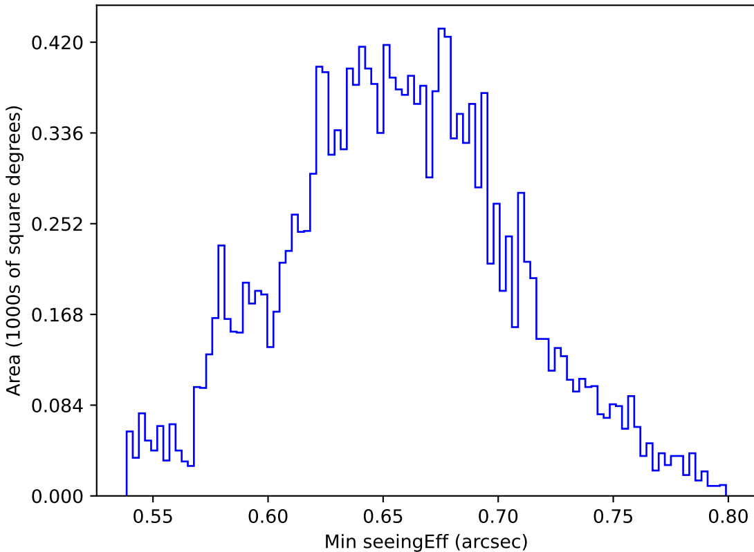
too_10_4v3.4_10yrs WFD g band: Min seeingEff
