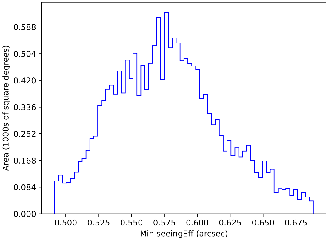
too_10_4v3.4_10yrs WFD all bands: Min seeingEff
