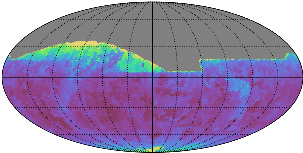
too_10_4v3.4_10yrs All sky z band: Min seeingEff
