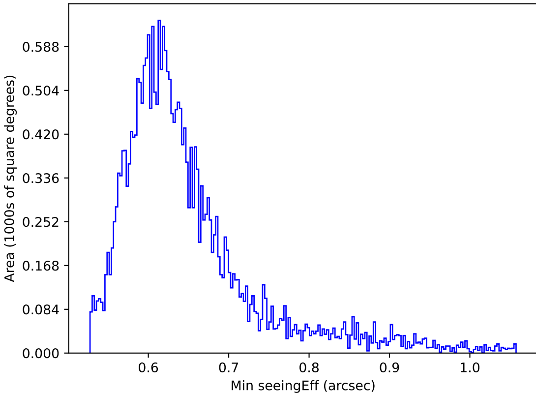
too_10_4v3.4_10yrs All sky z band: Min seeingEff
