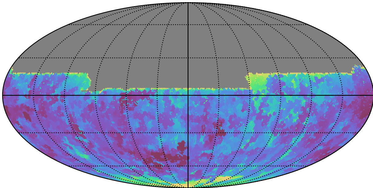
too_10_4v3.4_10yrs All sky u band: Min seeingEff
