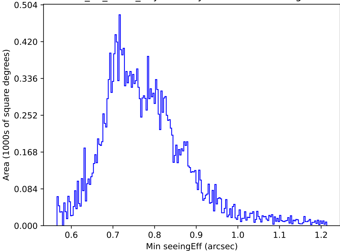
too_10_4v3.4_10yrs All sky u band: Min seeingEff
