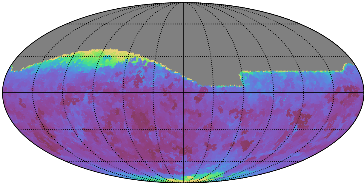
too_10_4v3.4_10yrs All sky r band: Min seeingEff
