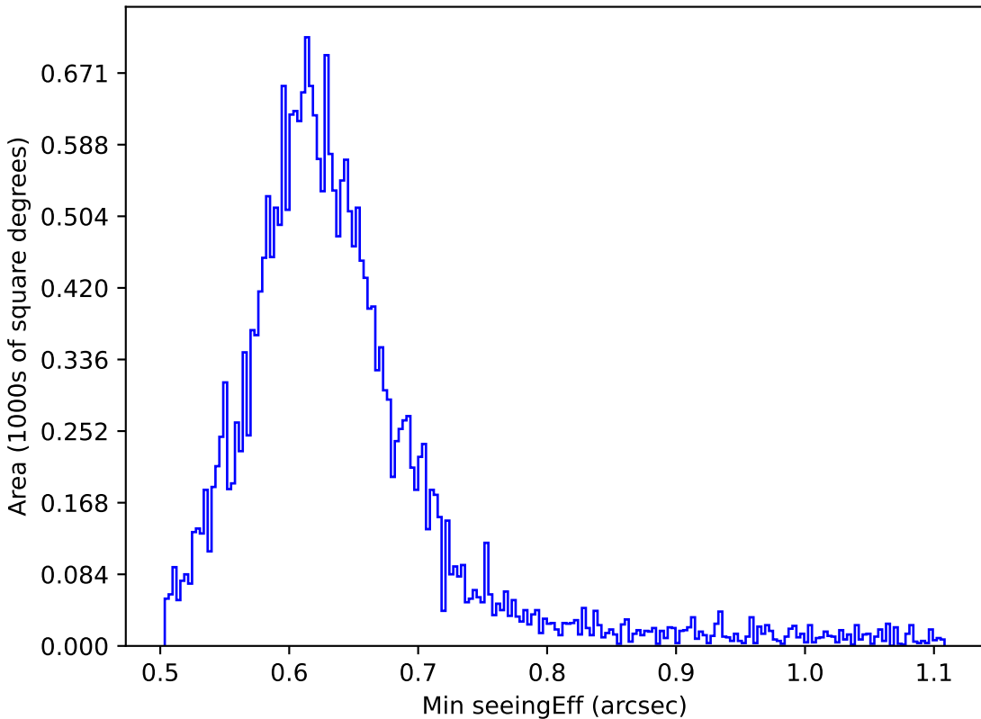
too_10_4v3.4_10yrs All sky r band: Min seeingEff
