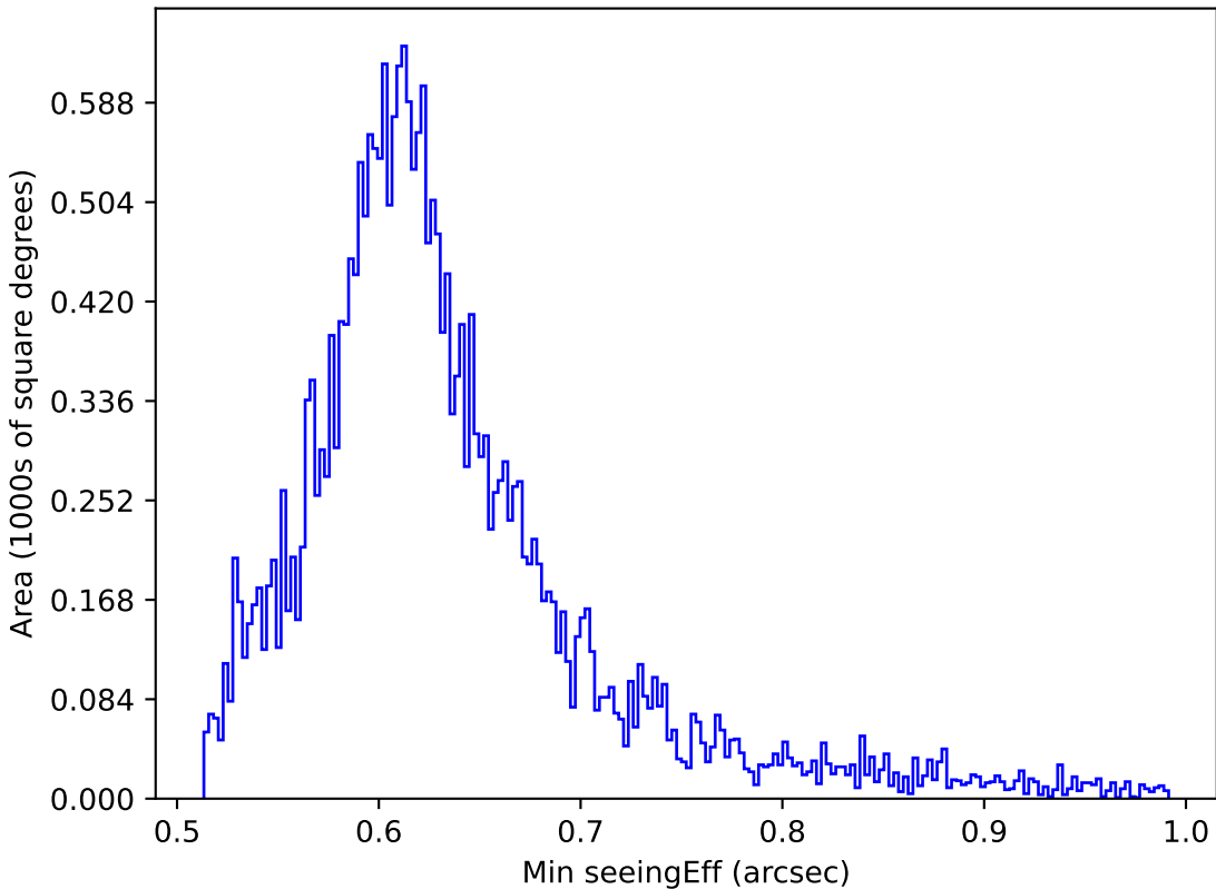
too_10_4v3.4_10yrs All sky i band: Min seeingEff
