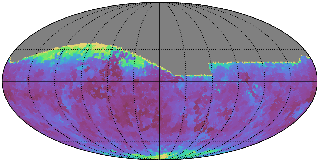
too_10_4v3.4_10yrs All sky g band: Min seeingEff
