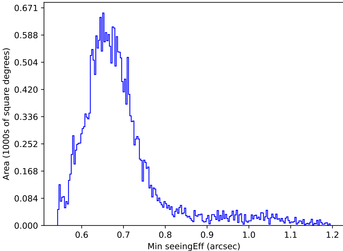
too_10_4v3.4_10yrs All sky g band: Min seeingEff
