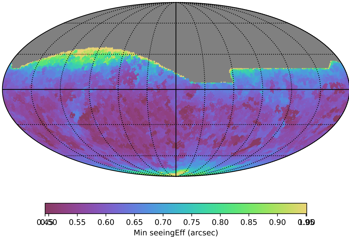
too_10_4v3.4_10yrs All sky all bands: Min seeingEff
