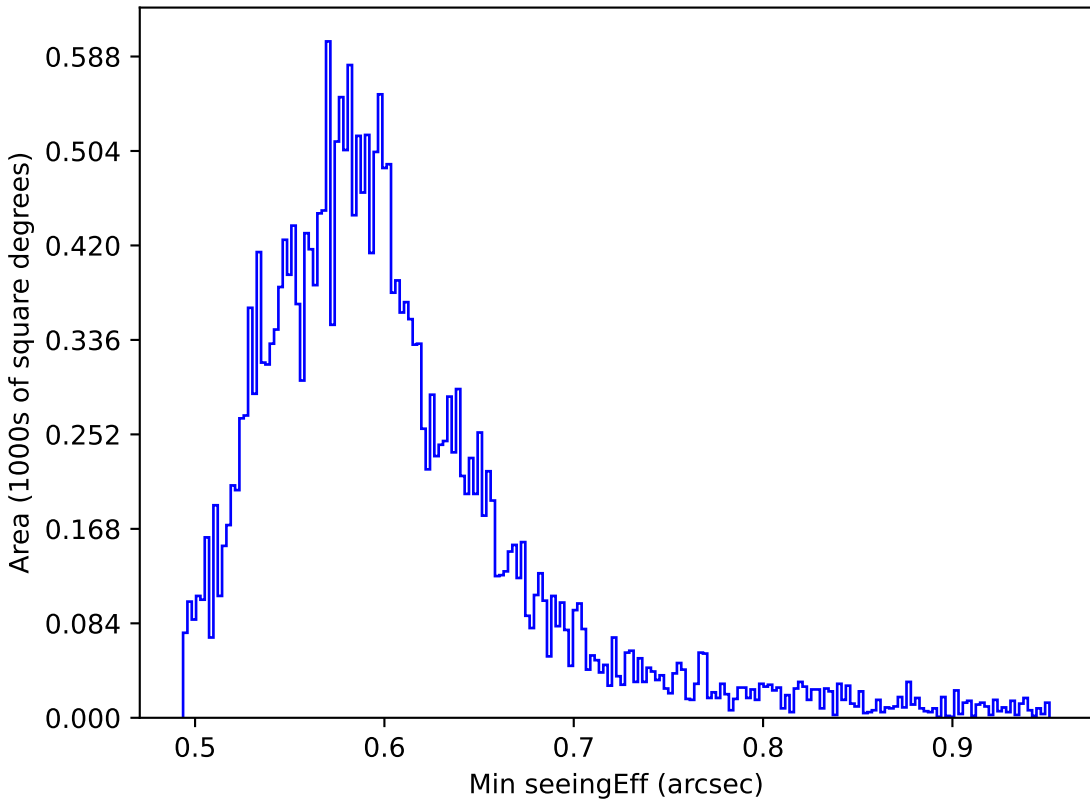
too_10_4v3.4_10yrs All sky all bands: Min seeingEff
