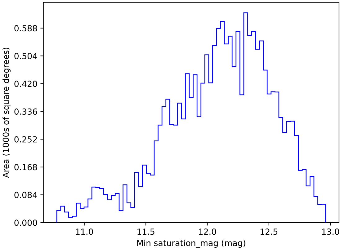
too_10_4v3.4_10yrs WFD z band: Min saturation_mag
