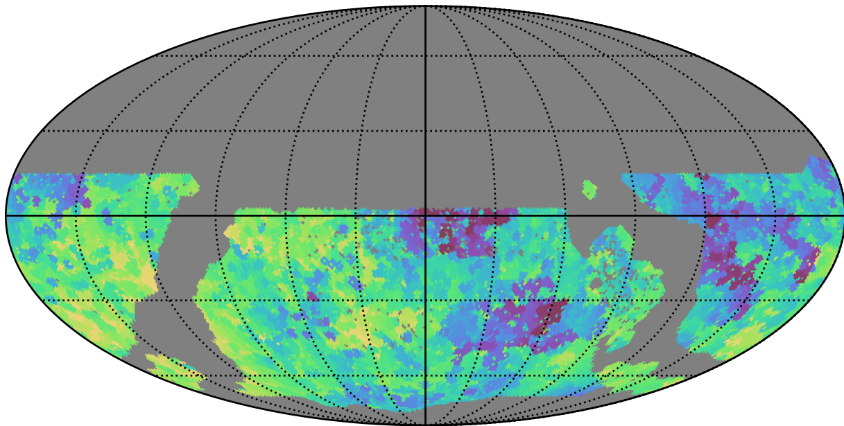
too_10_4v3.4_10yrs WFD y band: Min saturation_mag
