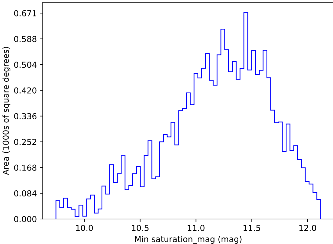
too_10_4v3.4_10yrs WFD y band: Min saturation_mag
