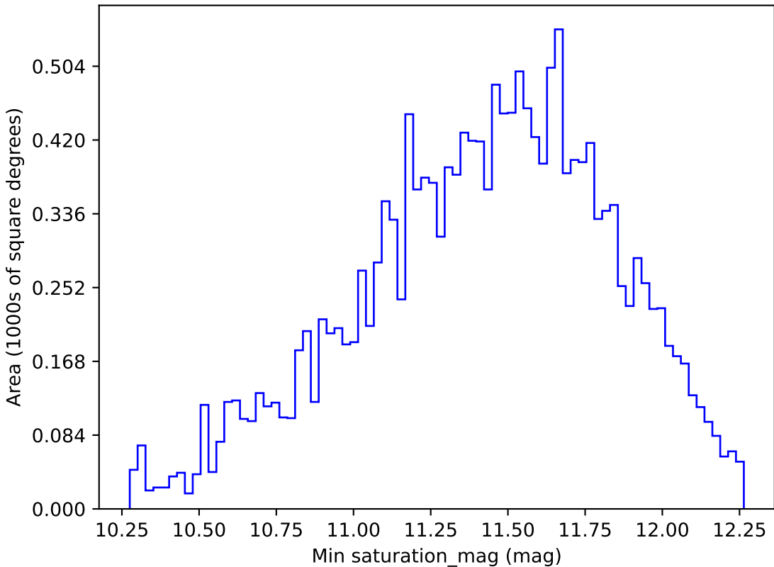
too_10_4v3.4_10yrs WFD u band: Min saturation_mag
