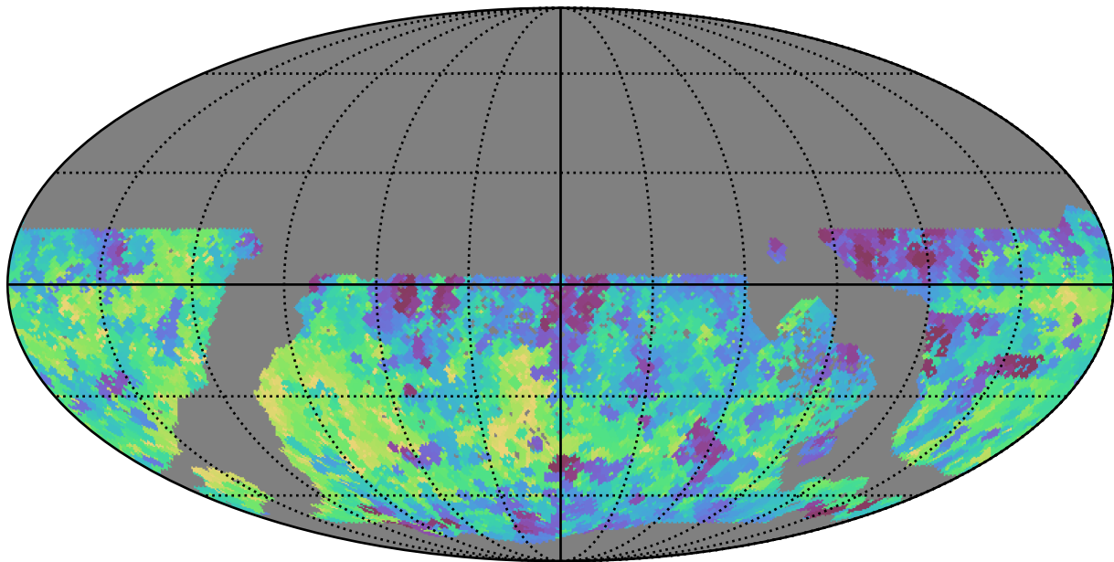
too_10_4v3.4_10yrs WFD r band: Min saturation_mag
