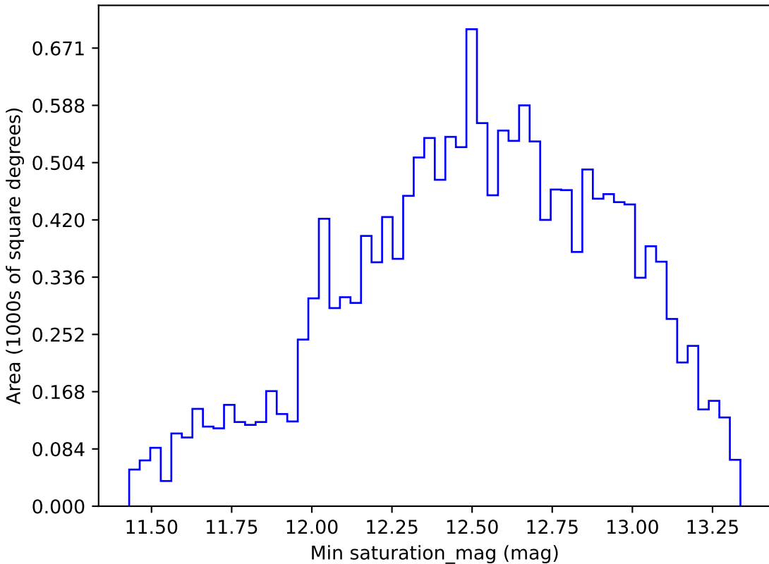
too_10_4v3.4_10yrs WFD r band: Min saturation_mag
