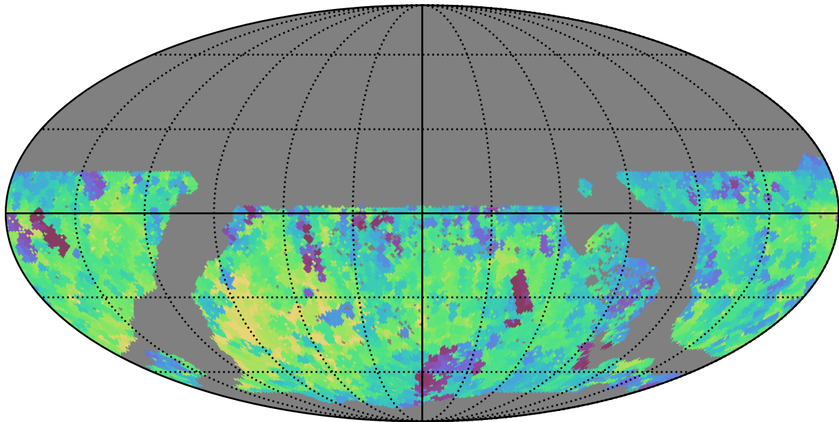
too_10_4v3.4_10yrs WFD i band: Min saturation_mag
