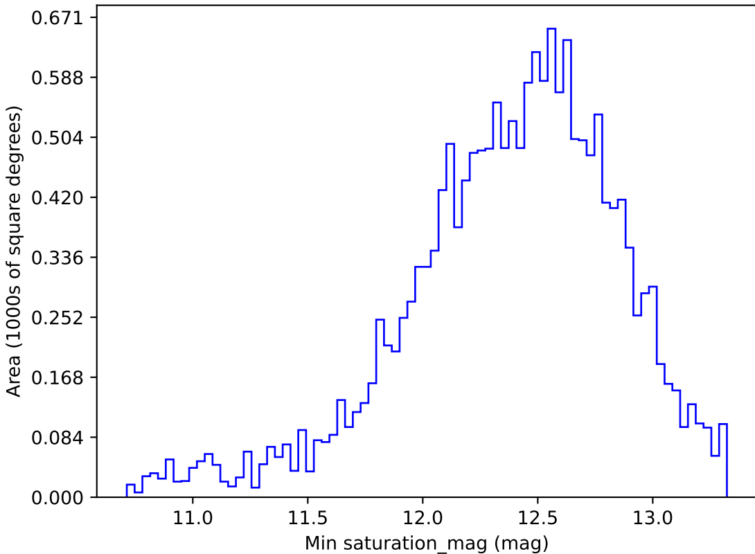
too_10_4v3.4_10yrs WFD i band: Min saturation_mag
