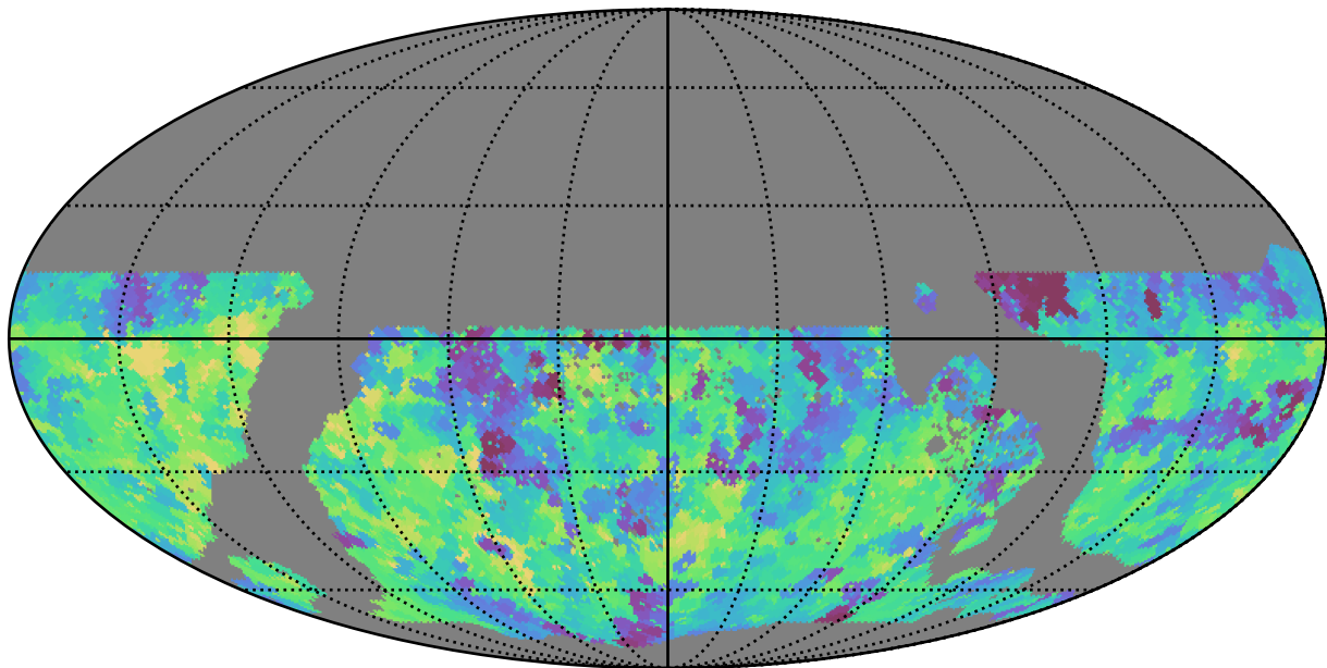
too_10_4v3.4_10yrs WFD g band: Min saturation_mag
