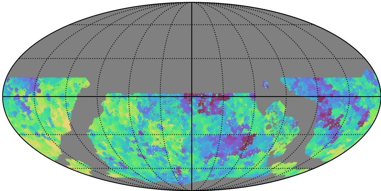
too_10_4v3.4_10yrs WFD all bands: Min saturation_mag
