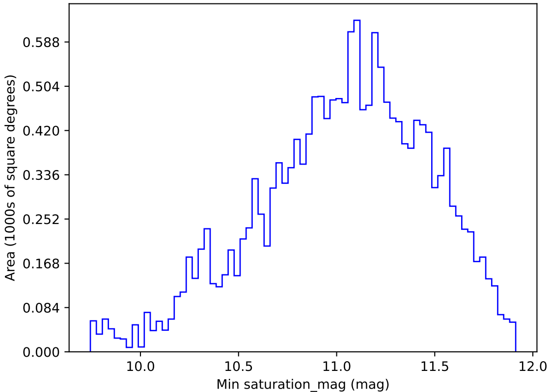
too_10_4v3.4_10yrs WFD all bands: Min saturation_mag
