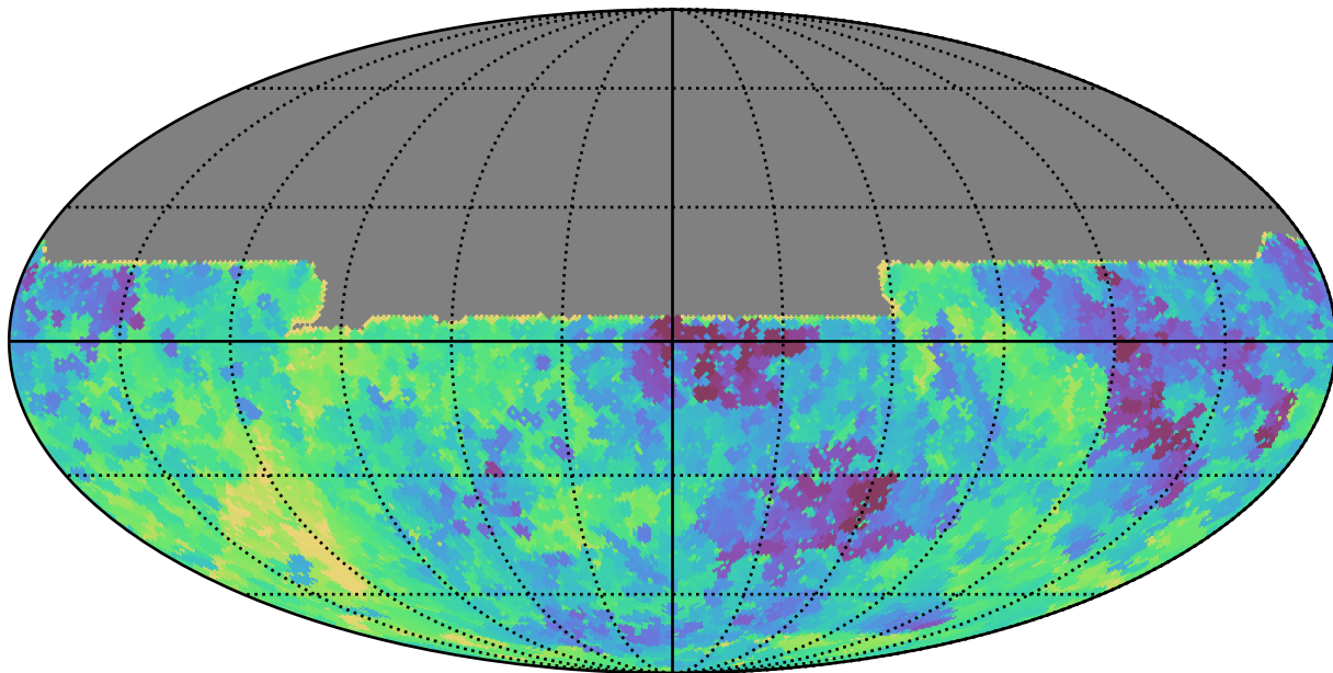
too_10_4v3.4_10yrs All sky y band: Min saturation_mag
