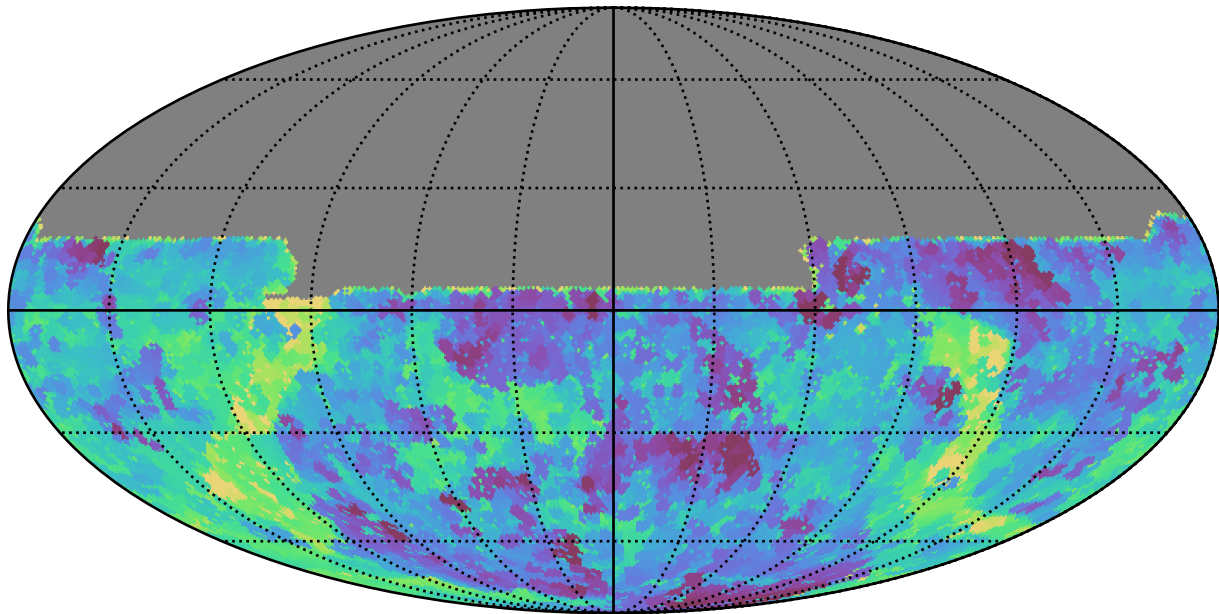
too_10_4v3.4_10yrs All sky u band: Min saturation_mag
