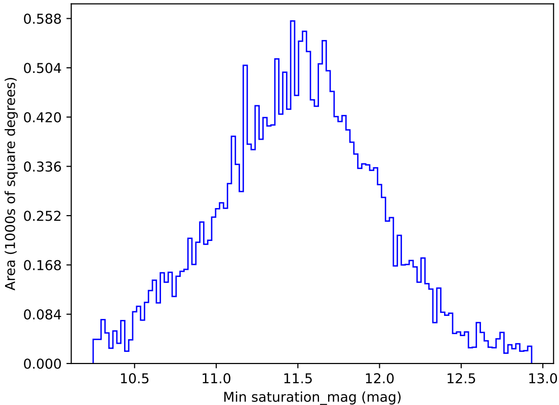
too_10_4v3.4_10yrs All sky u band: Min saturation_mag
