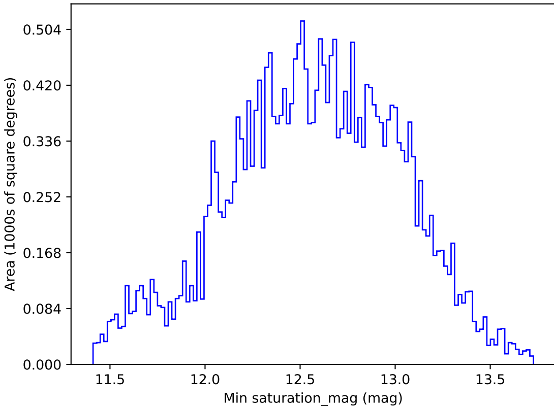
too_10_4v3.4_10yrs All sky r band: Min saturation_mag
