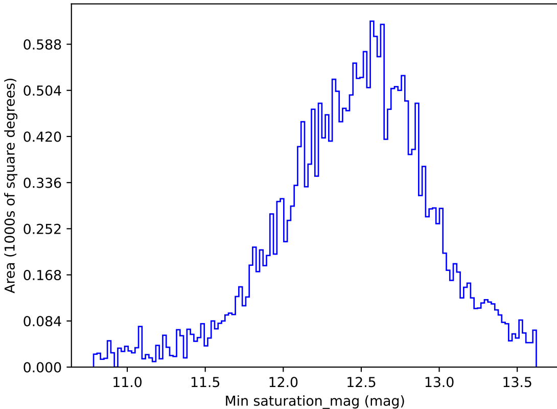
too_10_4v3.4_10yrs All sky i band: Min saturation_mag
