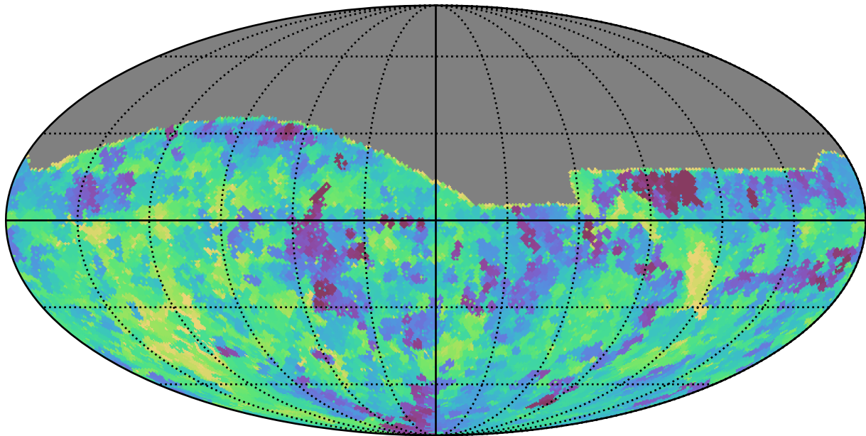
too_10_4v3.4_10yrs All sky g band: Min saturation_mag
