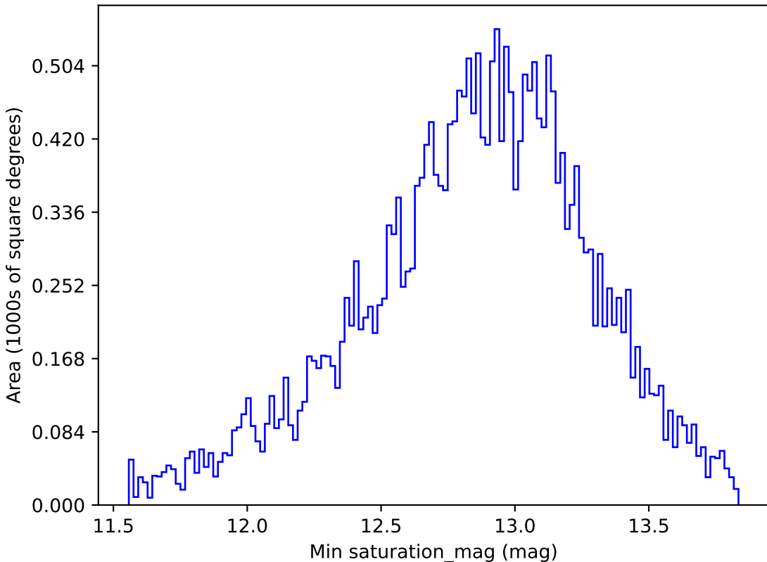
too_10_4v3.4_10yrs All sky g band: Min saturation_mag
