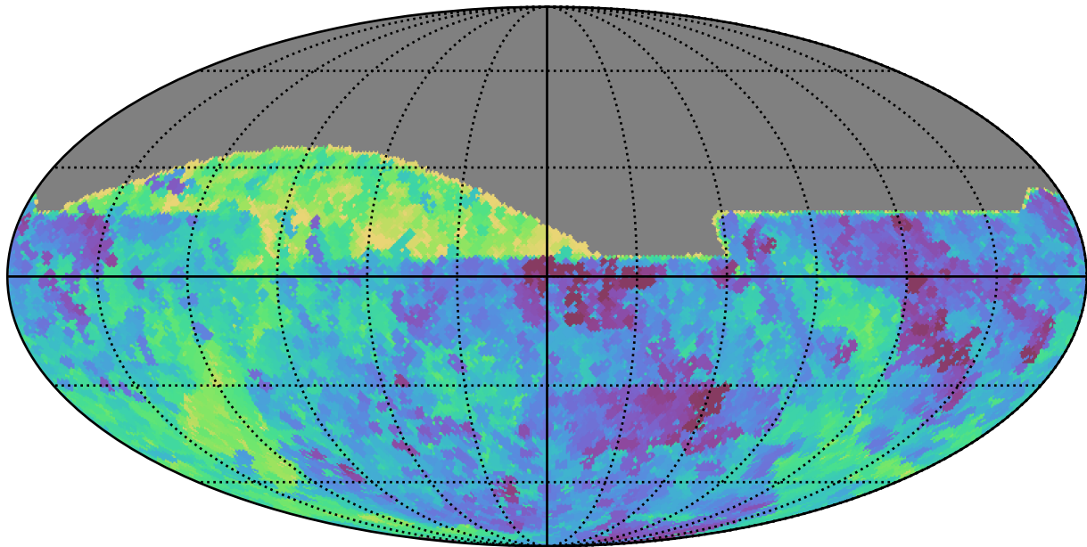
too_10_4v3.4_10yrs All sky all bands: Min saturation_mag
