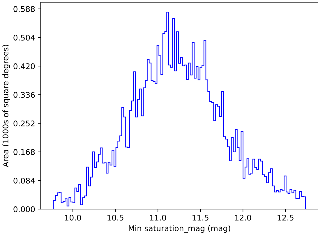
too_10_4v3.4_10yrs All sky all bands: Min saturation_mag
